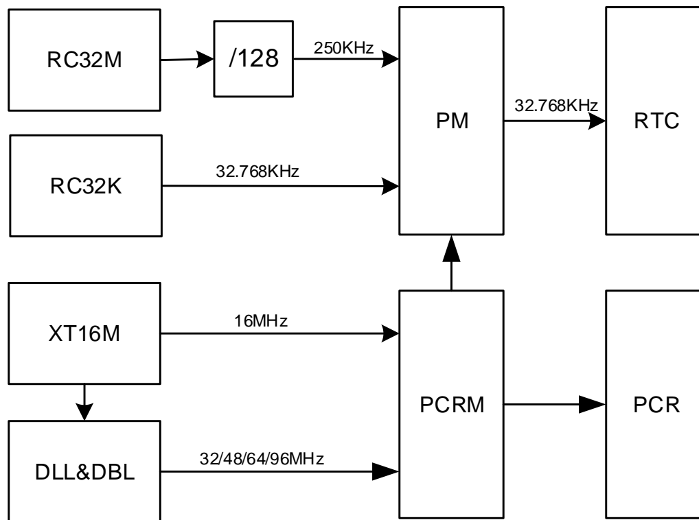
Figure 9: Clock management
