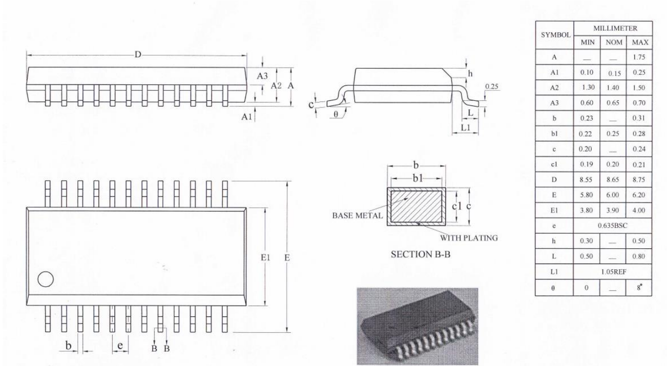
Figure 20: SSOP24 package dimensions
