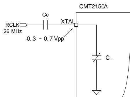
Figure 28. RCLK Circuitry
