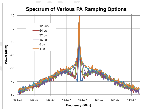
Figure 6. Spectrum of PA Ramping, SR = 9.6 kps, P_{OUT} = +10 dBm
