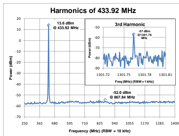
Figure 4. Harmonics of 433.92 MHz, P_{OUT} = +13 dBm
