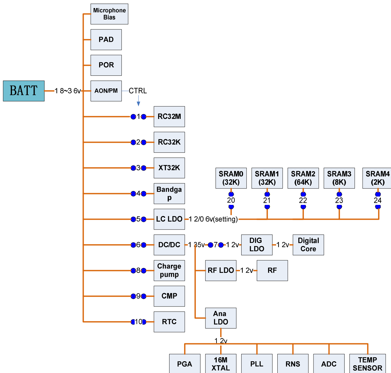
Figure 8: Power system
