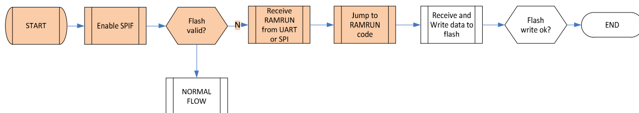
Figure6: Bootloader flow
