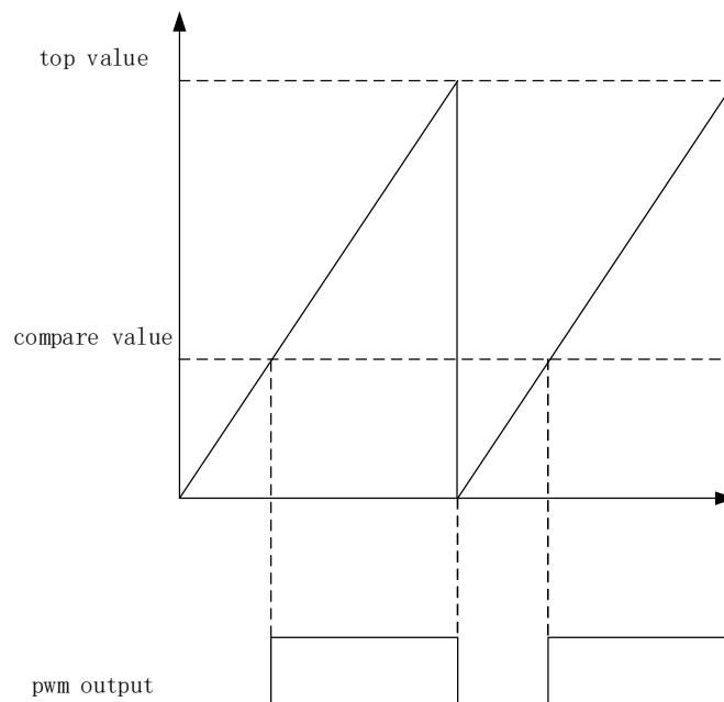
Figure13: PWM operation
