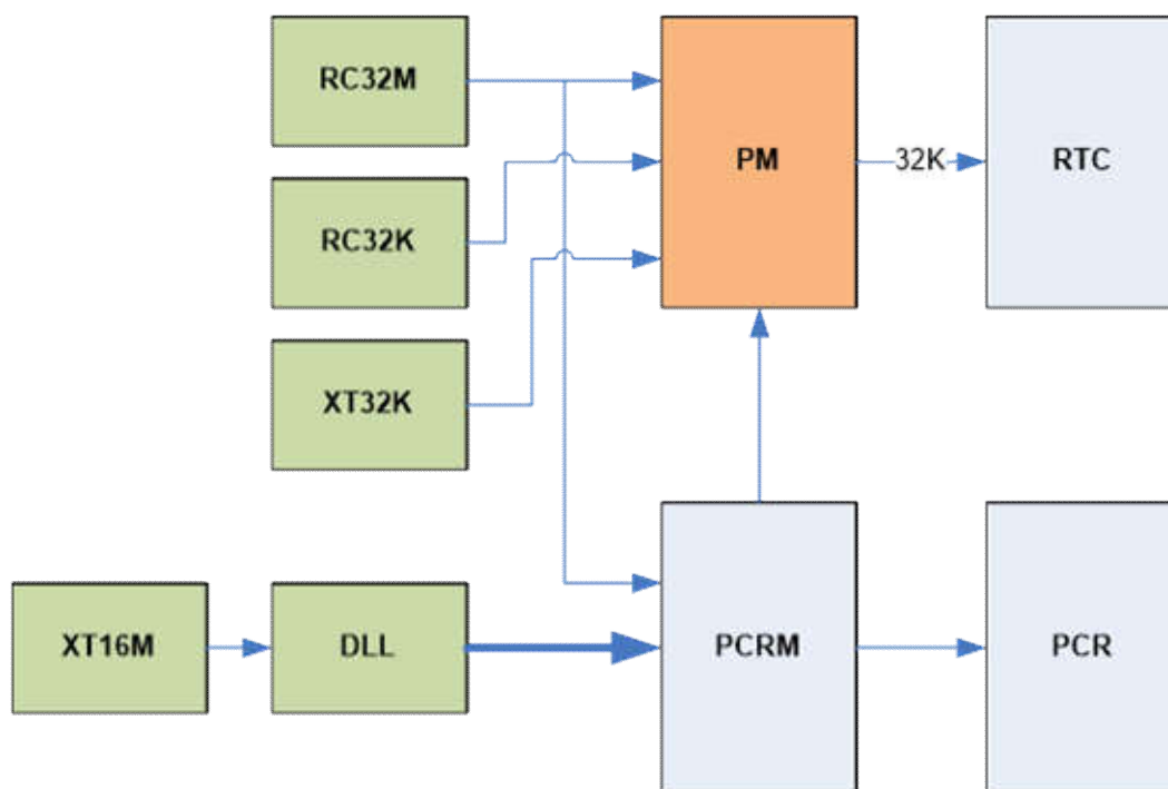
Figure 10: Clock management
